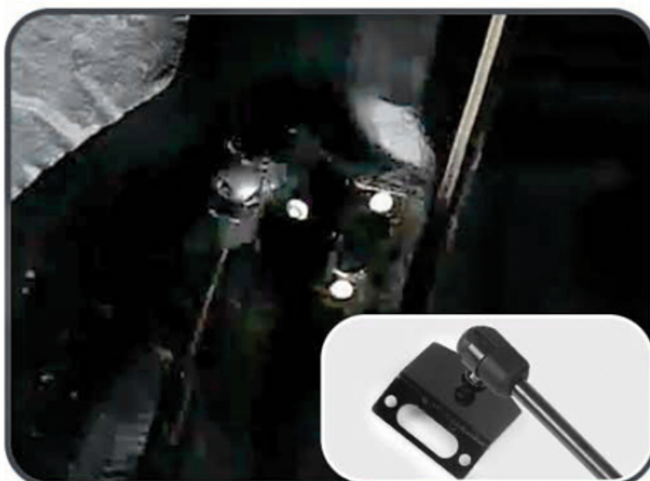
4. Mount the hood strut on the bracket
