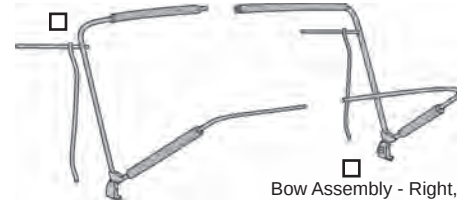
Bow Assembly - Left, Qty - 1, Part Number 385.99
